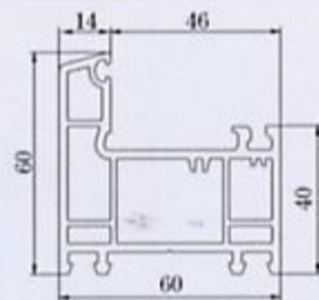
Frame-BR60
