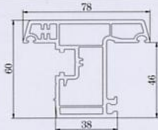
Outward Sash-SF78C
